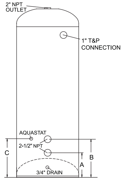
24" & 28" DIAMETER TANKS
